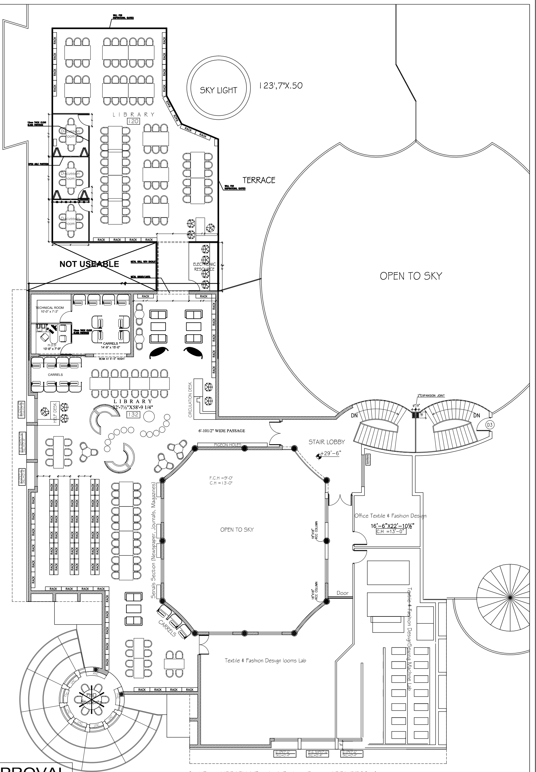
2nd Floor LIBRARY & Textile & Fashion Design AREA 5762 sft.
